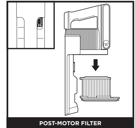
Remove the dust cup. Pull the post-motor filter out of the handheld vacuum.
